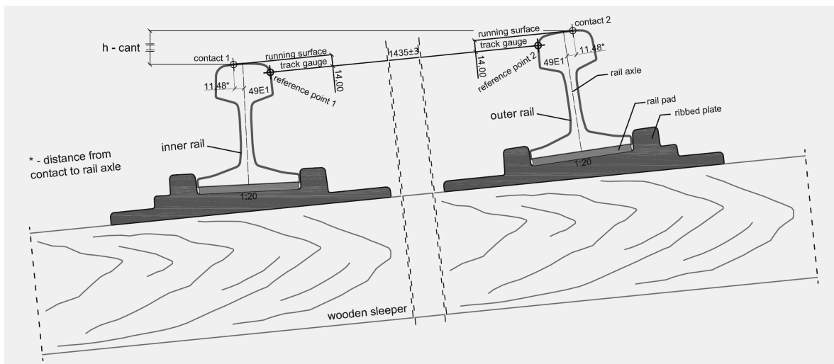
Figure 3. Initial position of track rails in curve without track widening
