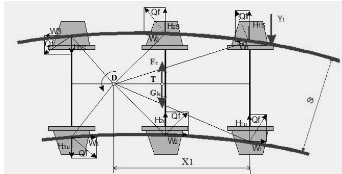
Figure 1. Inclined loose position of three axle bogie in curve (guiding force Y_1 that acts on the outer wheel of the first axle, lateral forces H_i and longitudinal friction forces W_i , centrifugal force F_c , weight G ) and current centre of rotation D
