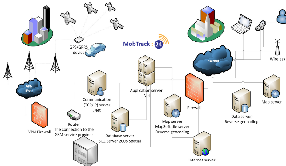
Figure 14. MobTrack:24 system architecture
