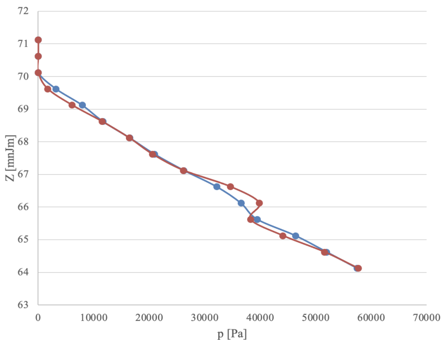
Slika 10. Raspored pritisaka po dubini za uzvodno i nizvodno lice nizvodne grupe odbojnika Figure 10. Pressure distribution along the upstream and downstream side of the downstream row of the plates
