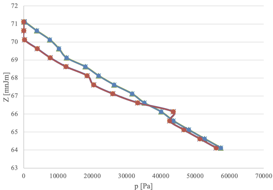
Slika 9. Raspored pritisaka po dubini za uzvodno i nizvodno lice uzvodne grupe odbojnika Figure 9. Pressure distribution along the upstream and downstream side of the upstream row of the plates
