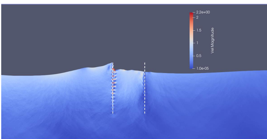
Slika 8. Prikaz fluidnih delića u zoni odbojnika 18 sekundi nakon početka simulacije Figure 8. Fluid particle level in the breakwater structure vicinity, 18 s after the start of the simulation
