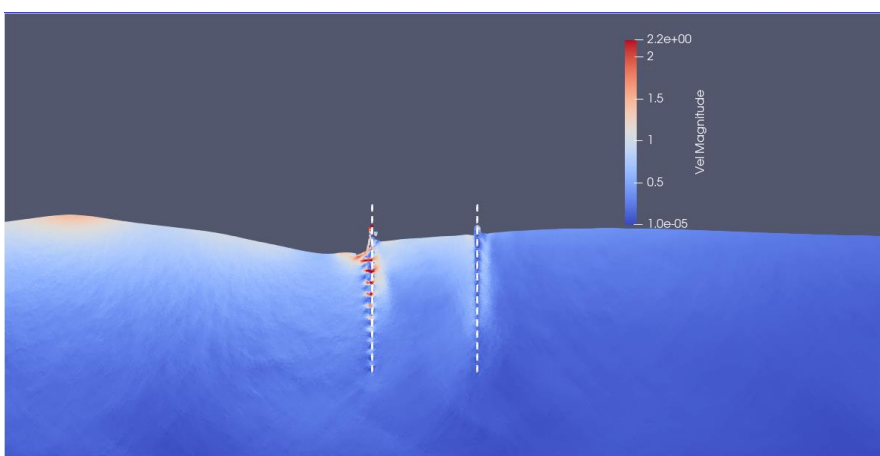
Slika 7. Prikaz fluidnih delića u zoni odbojnika 16 sekundi nakon početka simulacije Figure 7. Fluid particle level in the breakwater structure vicinity, 16 s after the start of the simulation
