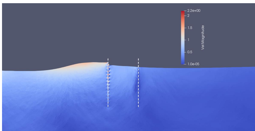
Slika 6. Prikaz fluidnih delića u zoni odbojnika 14 sekundi nakon početka simulacije Figure 6. Fluid particle level in the breakwater structure vicinity, 14 s after the start of the simulation
