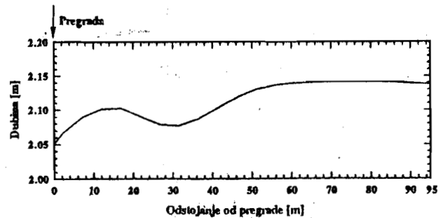
Sl. 6. - Uzdužni presek kroz osu vrtloga (presek b-b; t=2.3 min) Longitudinal cross section through the center-line of the vortex (cross section b-b; t=2.3 min)
