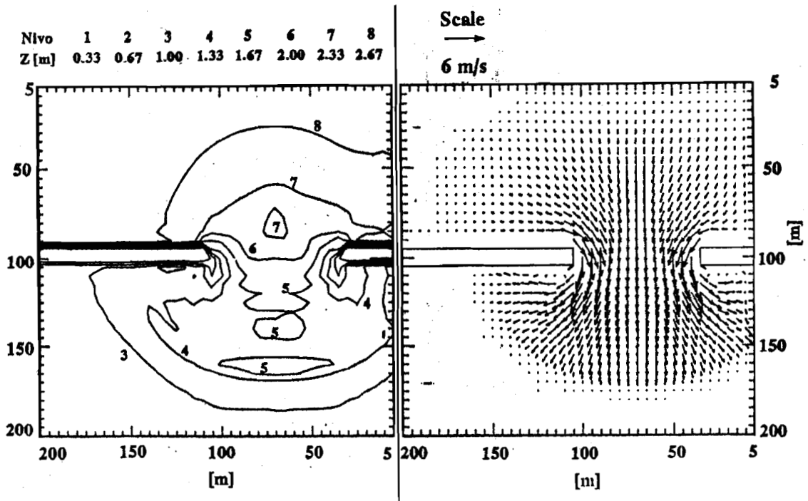
Sl. 3. - Prolom brane - izolije i polje brzine (t = 15 s) Dam break problem - contour lines and velocity field (t = 15 s)
