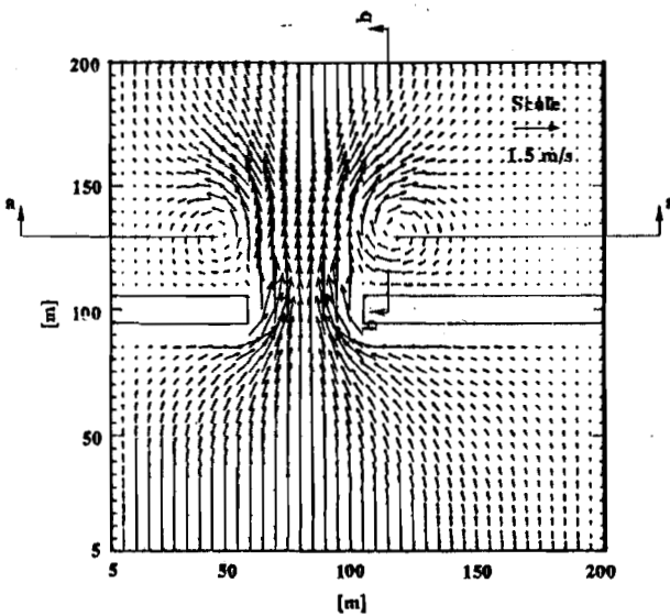
Sl. 4. - Ravansko tečenje kroz suženje (t=2.3 min) Two-dimensional flow through constriction (t=2.3 min)
