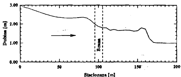
S1. 2. – Prolom brane - uzdužni profil po osovini otvora ( t=15 s) Dam break problem - longitudinal water surface profile ( t + 15 s)
