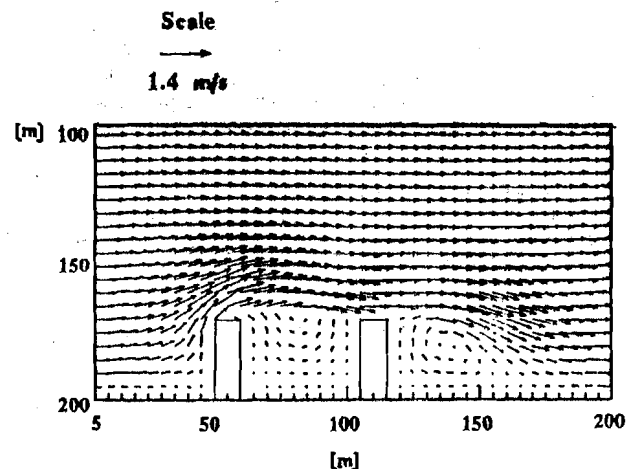
Sl. 8. – Strujna slika u blizini dva napera ( t=4.3 min) Flow field in the vicinity of two groynes ( t=4.3 min)
