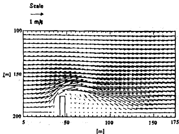
Sl. 7. – Strujna slika u blizini jednog napera ( t=4.5 min) Flow field in the vicinity of a groyne ( t=4.5 min)
