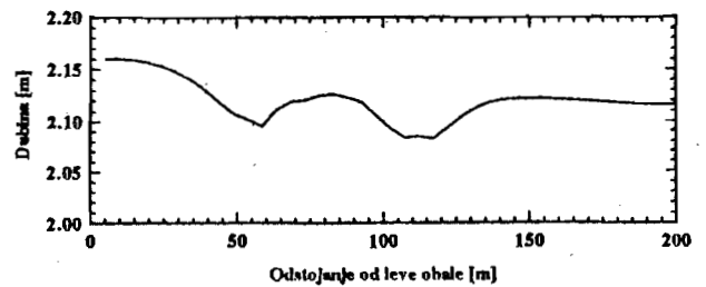
Sl. 5. - Poprečni presek kroz osu vrtlogâ (presek a-a; t=2.3 min) Cross section through the center-line of the vortices (cross section a-a; t=2.3 min)
