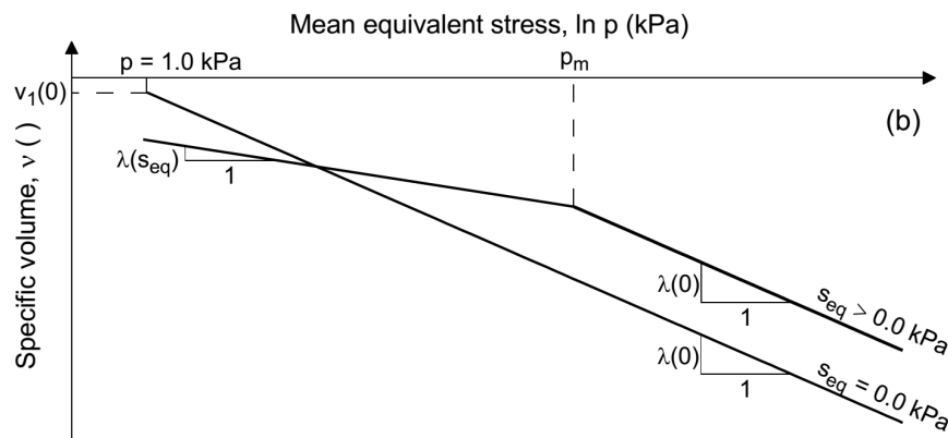
Figure 3.19 Bi-linear unsaturated isotropic compression line (ICL), after (Georgiadis, 2003)
