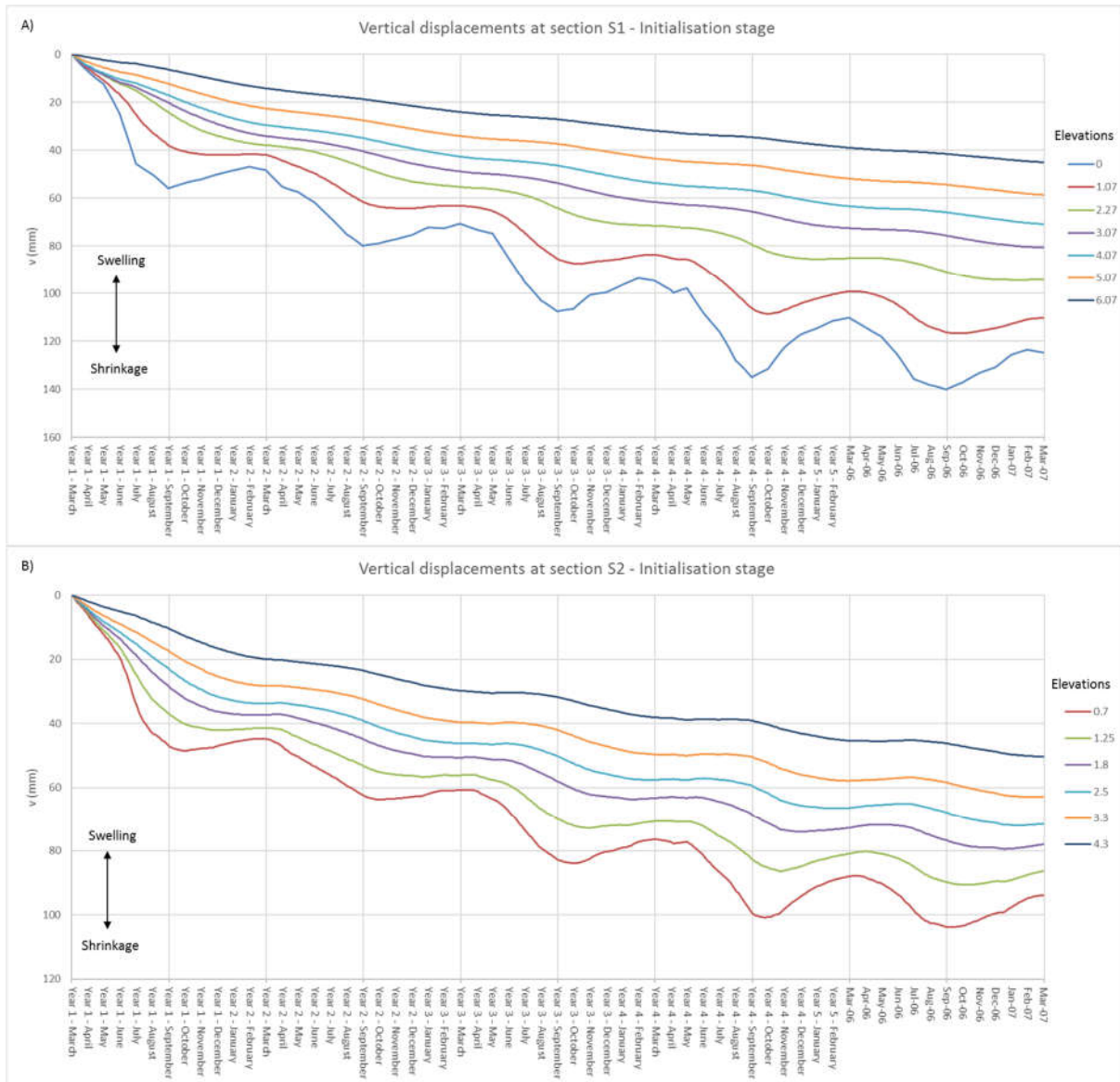
Figure 4.32 Predicted vertical displacements at sections S1 and S2 of the north-facing embankment slope
