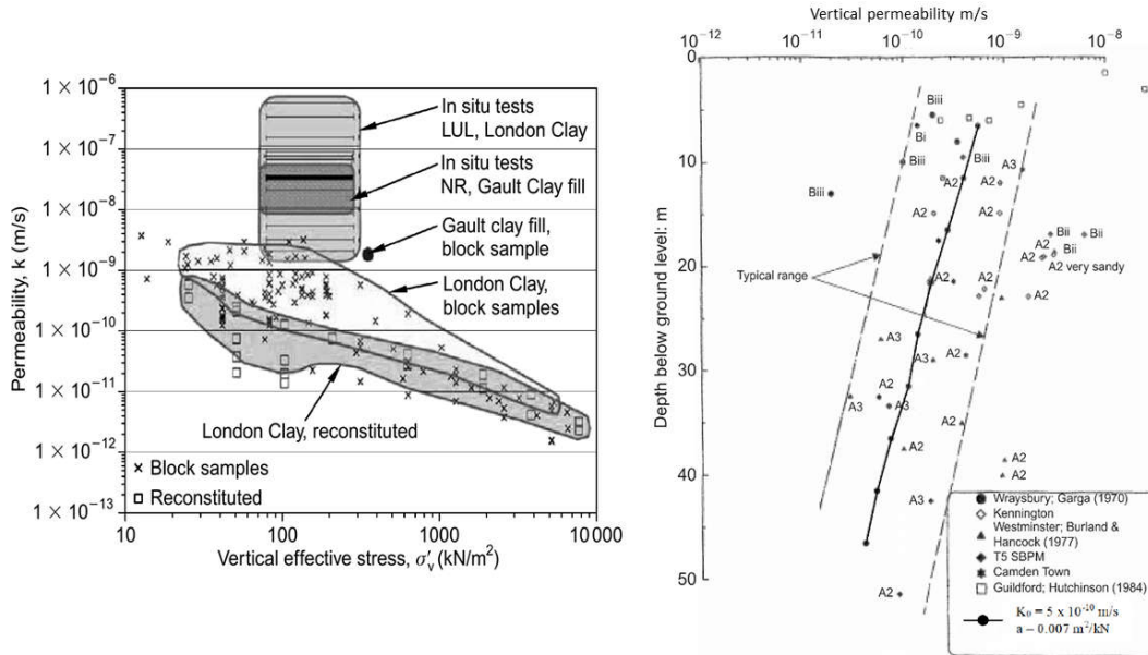
Figure 4.15 Permeability data for A) dumped clay fill (O'Brien, 2013) and B) London Clay from in situ tests (Hight et al., 2003)
