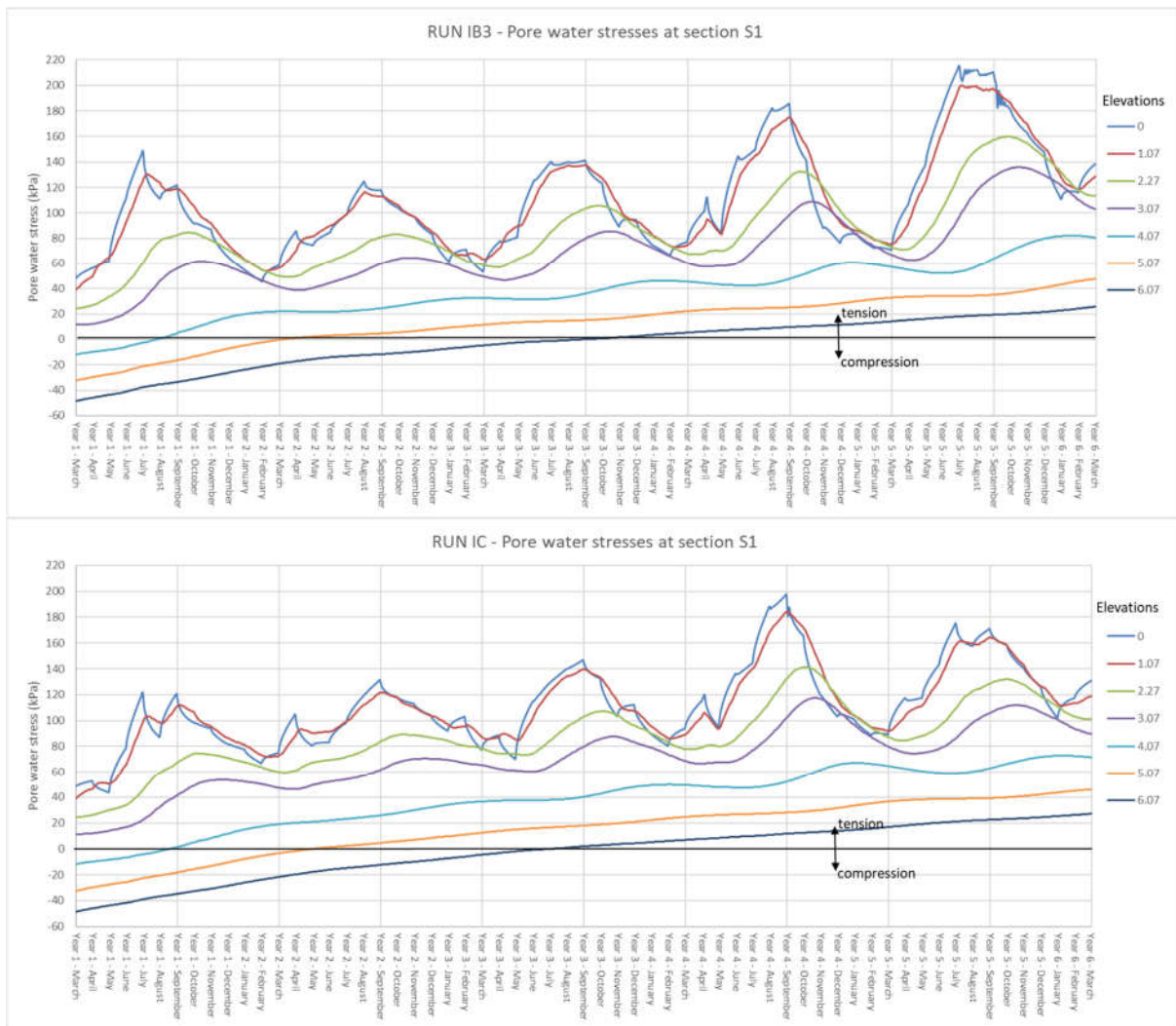
Figure 5.6 Predicted seasonal pore water pressure variations for two different evapotranspiration data sets (top-Mat Office, bottom-Thornthwaite)
