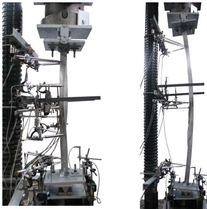
(a) ACF 80 \times 80 \times 4 - 1000 - 4
