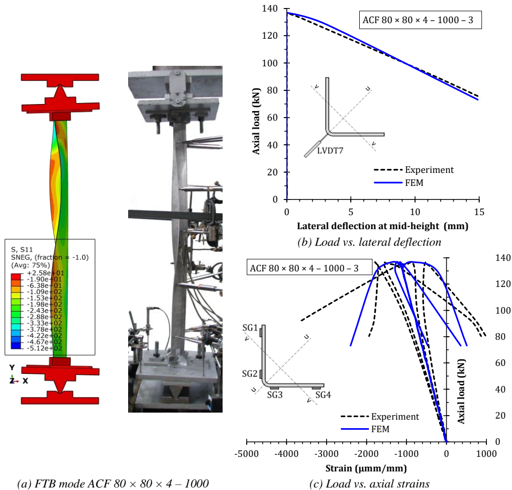
Figure 3 - FE model and experimental buckling mode of intermediate length specimens [2]
