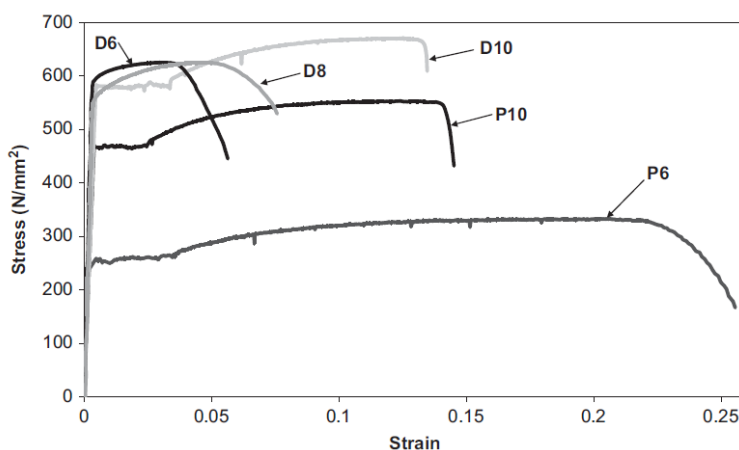
Figure 1. Results of tensile test in room temperature [3]
