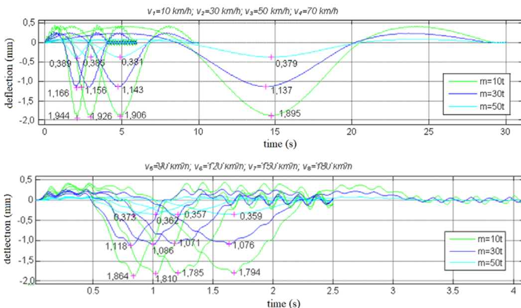
Figure 4. Deflections in the middle of the span at different time intervals for model 1, speeds of 10-180 km/h
