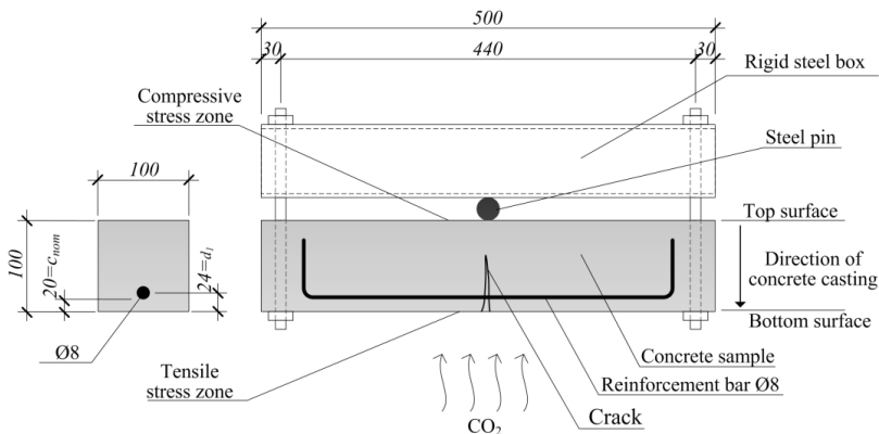
Figure 1. Experiment setup.
