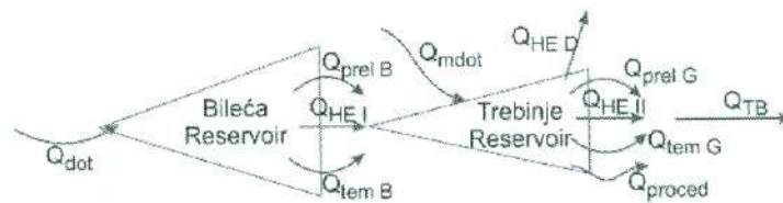
Figure 4. Schematic view of Trebišnjica Hydrosystem (I phase)
