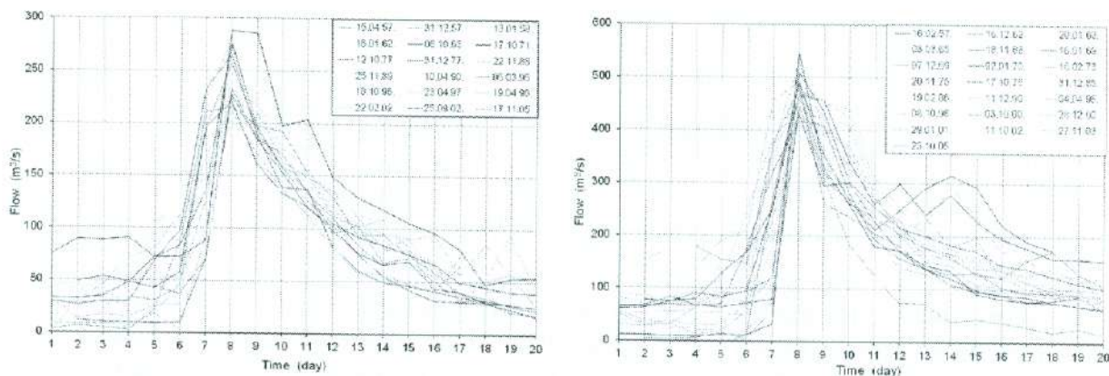
Figure 3. Medium and high flood waves for Bileća Reservoir
