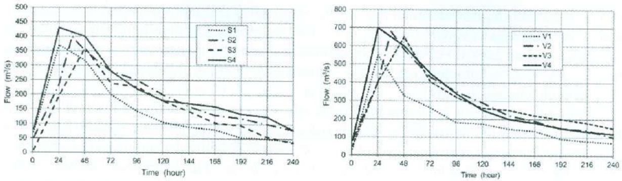
Figure 5. Synthetic flood waves for Bileća Reservoir
