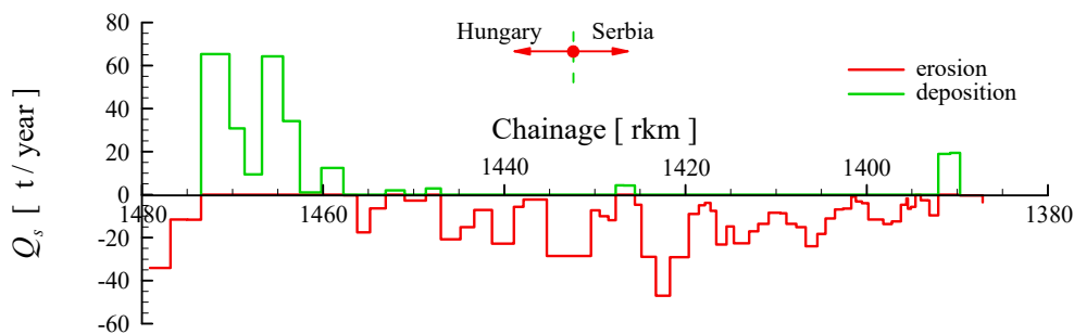
Figure 11. Twenty-five-year long-term changes in sediment transport with sediment deposition and erosion patterns.
