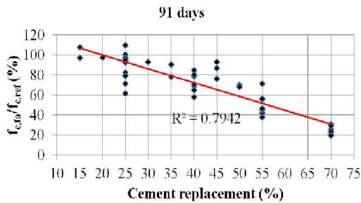
Figure 3. Compressive strenght of fly ash concrete/compressive strenght of cement concrete ratio at the age of 91 days depending on the cement replacement [17, 18, 19, 20, 21]
