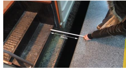
Fig.4. The unsafe gap in the Vukov Spomenik railway station in downtown Belgrade
