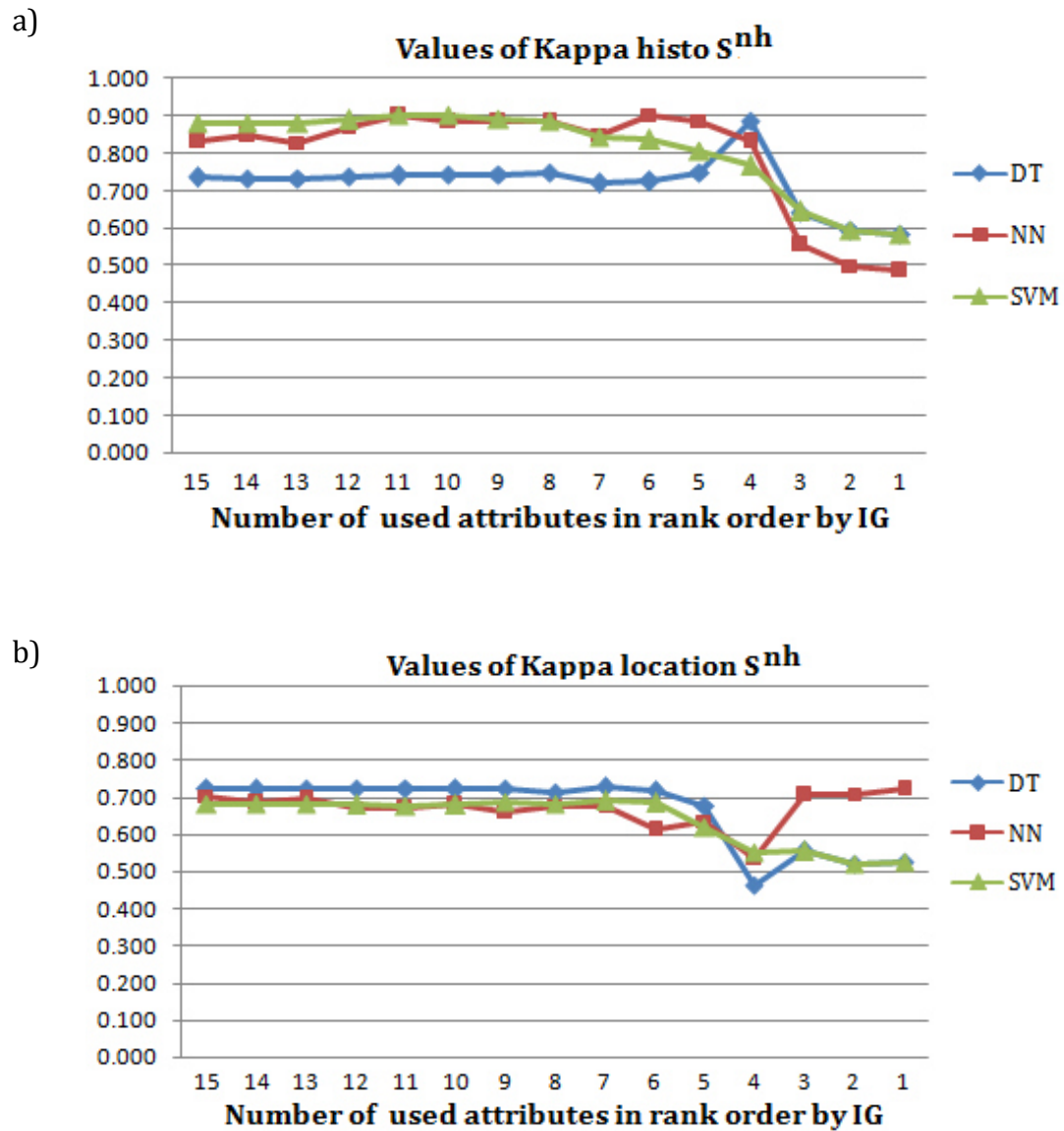
Figure 5.7 Obtained values of a) kappa histo and b) kappa location in a recursive attribute elimination process using attributes from S^{nh} ranked by IG.
