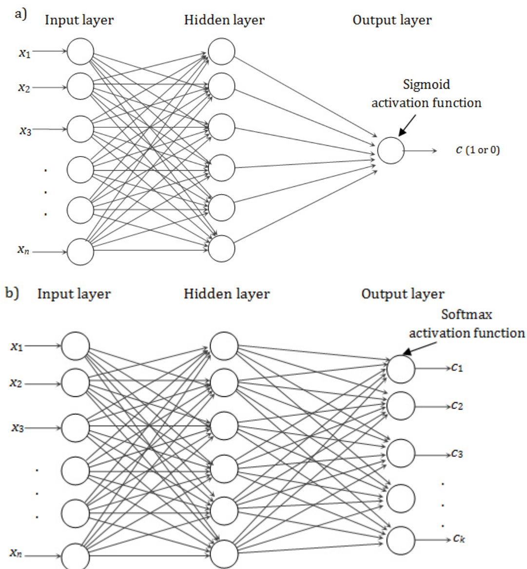
Figure 3.6 Schematic representation of a MLP classification network for a) two classes and b) k -classes, k > 2 .
