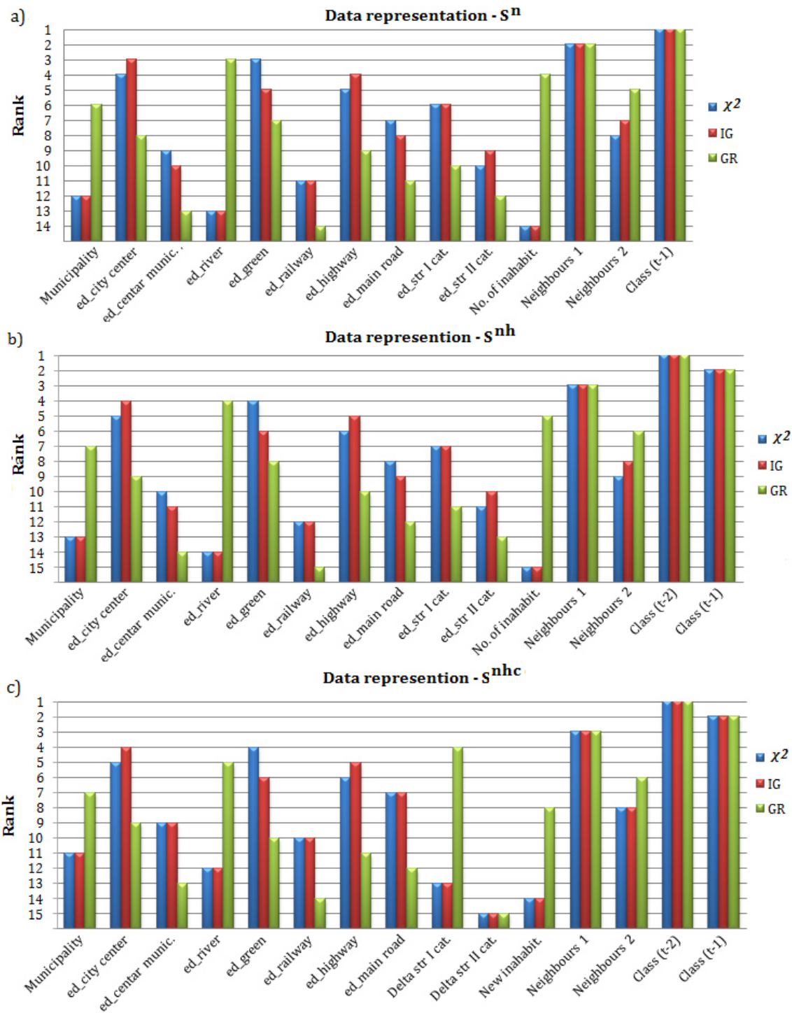
Figure 5.4 Attribute ranking values based on \chi^2 , IG and GR method for data representation a) S^n , b) S^{nh} and c) S^{nhc} .
