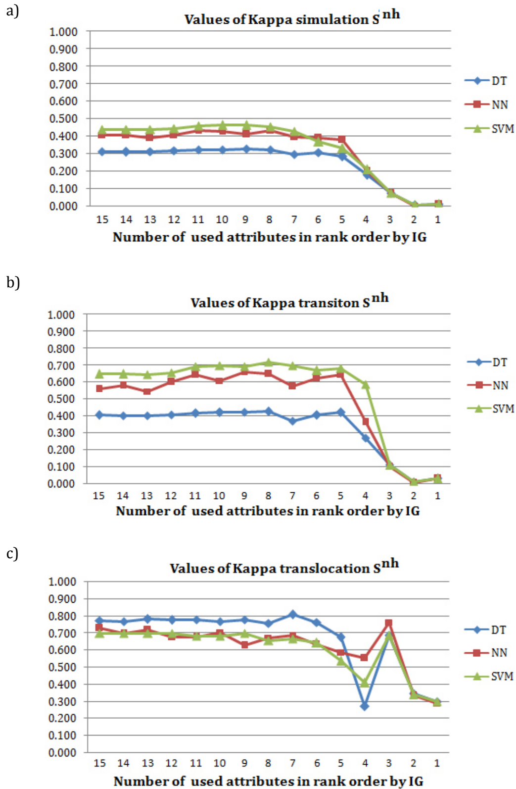
Figure 5.8 Obtained values of a) kappa simulation b) kappa transition and c) kappa transloc in a recursive attribute elimination process using attributes from S^{nh} ranked by IG.
