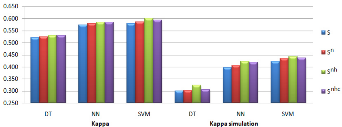
Figure 5.2 Comparison of the validation measures of models for four data representations S , S^n , S^{nh} , and S^{nhc} for all three machine learning techniques.
