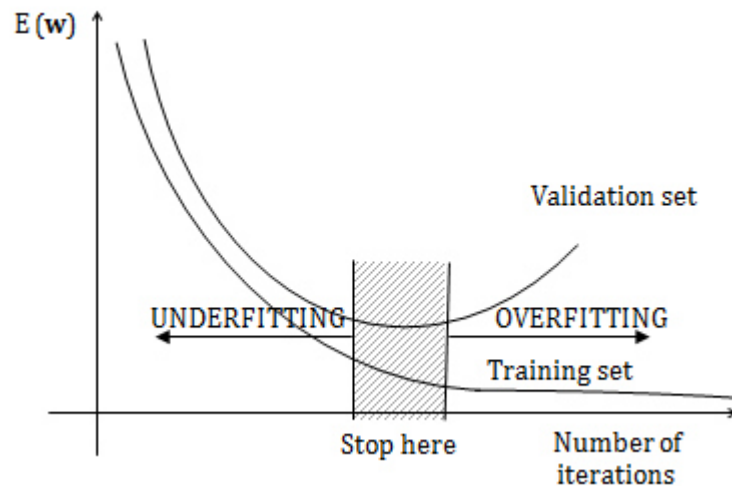
Figure 3.7 Stop criteria for training NN using validation and training sets.
