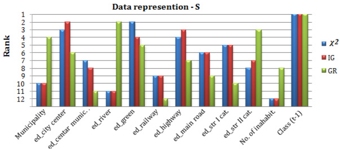
Figure 5.3 Attribute ranking values based on \chi^2 , IG and GR method for data representation S.
