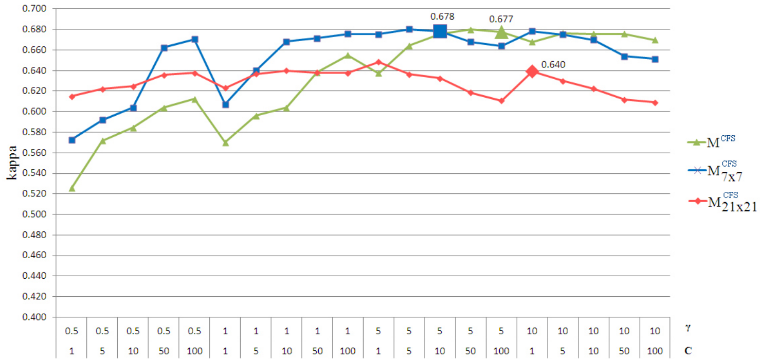
Figure 5.18 Comparison of the model performance derived with different data representation and different values of SVM parameters C and \gamma .
