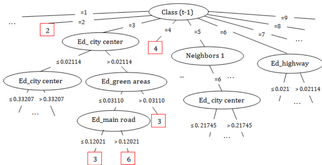
Figure 5.9 Part of the built decision tree for S^{nh} data representation.
