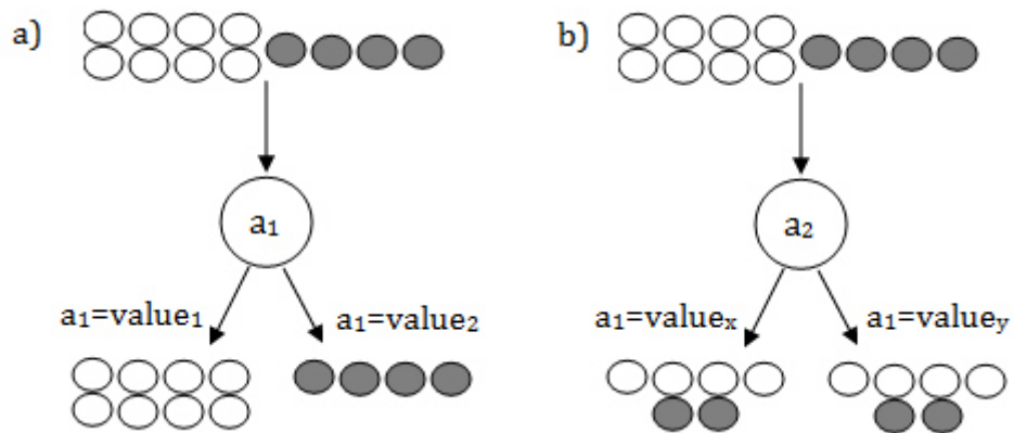
Figure 3.3 Choosing the attribute in the internal node of the growing tree; a) perfect attribute choice, b) the worst attribute choice.
