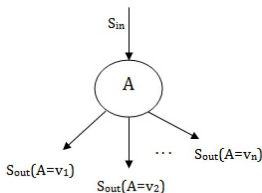
Figure 3.4 Calculating Gain Ratio of an attribute in the internal node of the growing tree.
