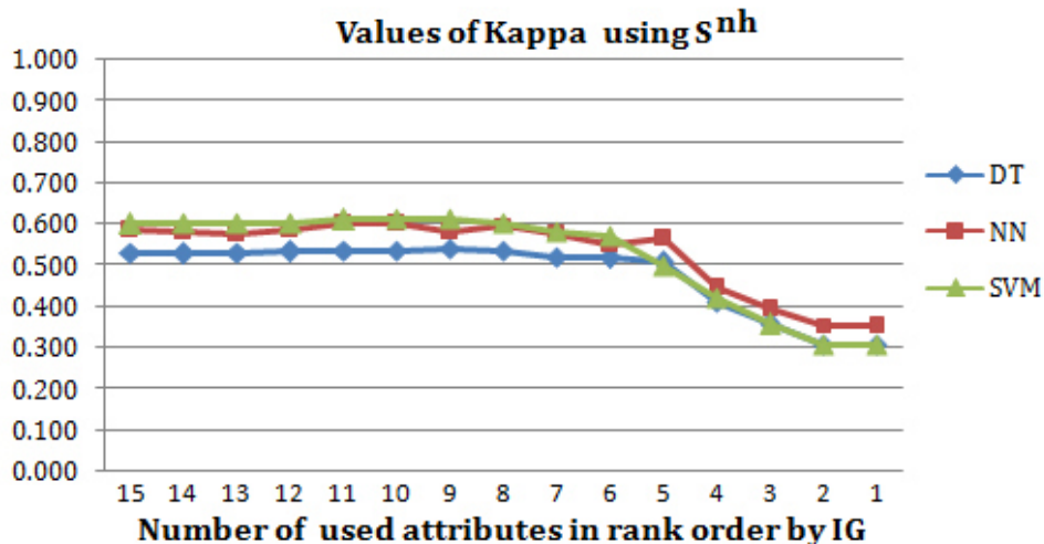
Figure 5.5 Obtained values of kappa in a recursive attribute elimination process using attributes from S^{nh} ranked based on IG.
