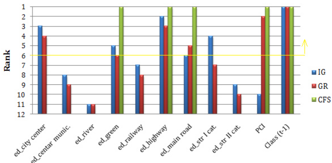
Figure 5.16 Selection of attributes by IG, GR and CFS.
