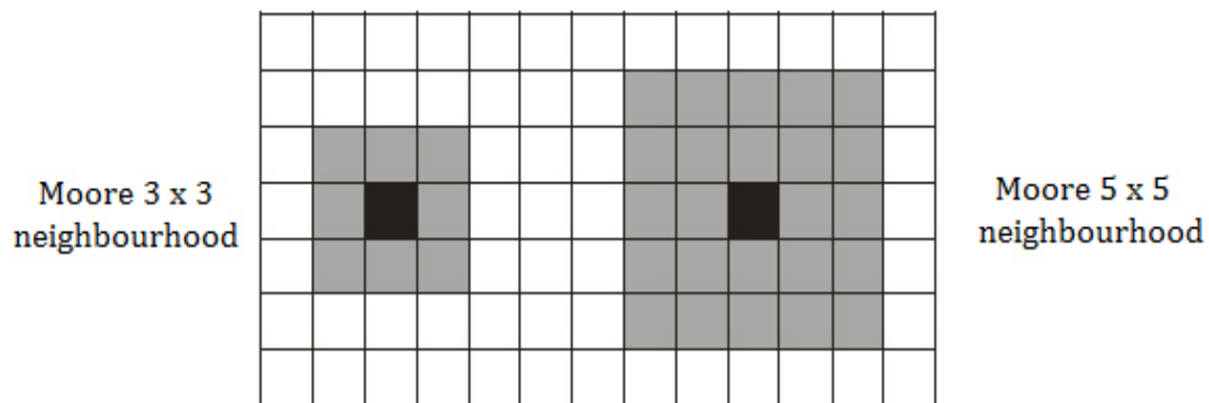
Figure 4.9 Moore neighbourhoods.
