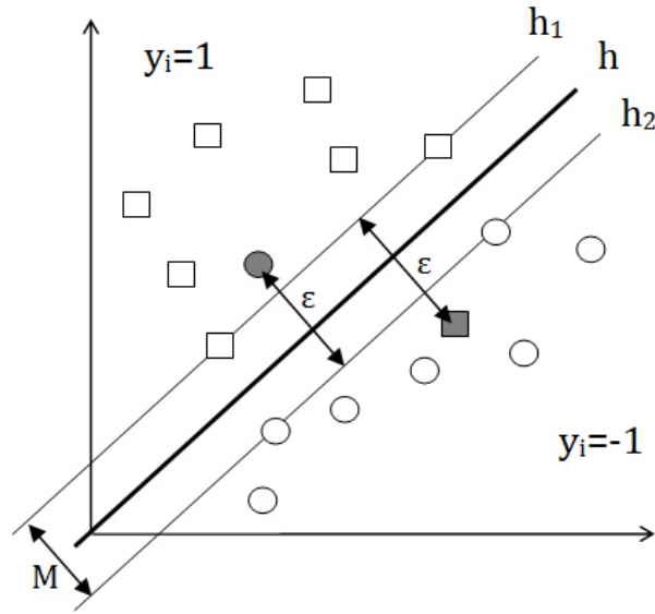
Figure 3.8 General binary classification case ( h: \mathbf{w}\mathbf{x}+b=0 ; h_1: \mathbf{w}\mathbf{x}+b=1 ; h_2: \mathbf{w}\mathbf{x}+b=-1 ). Shaded points \varepsilon represent misclassified instances.
