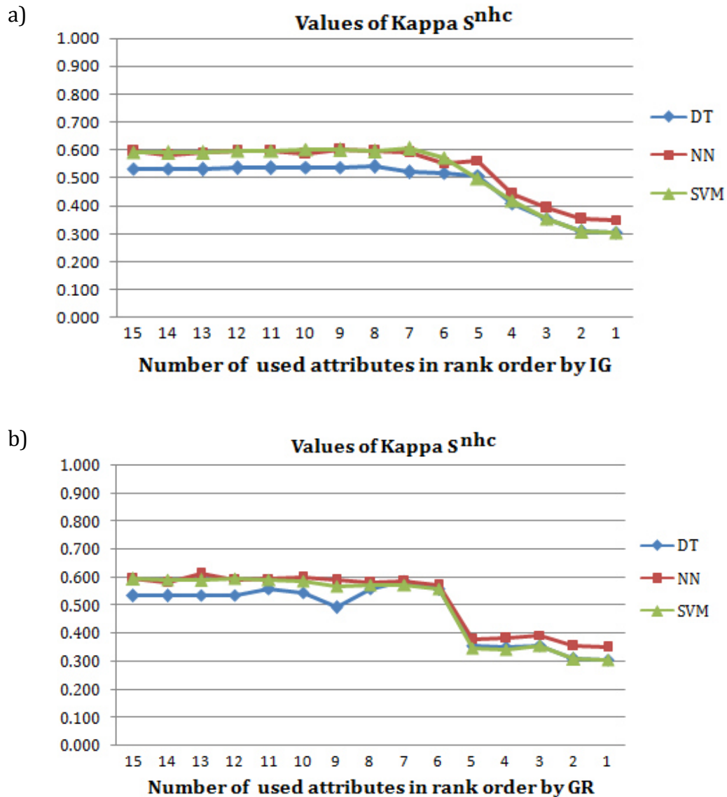
Figure 5.6 Obtained values of kappa in a recursive attribute elimination process using attributes from S^{nhc} ranked based on a) IG and b) GR.
