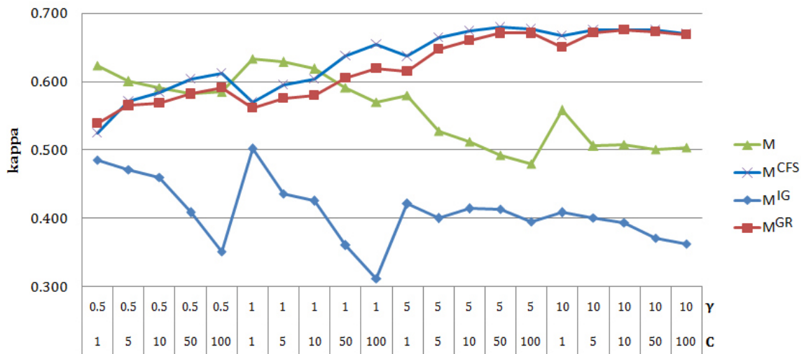
Figure 5.17 Comparison of the model performance derived with all attributes (M) and with subset of 5 selected attributes based on the CFS ( M^{CFS} ), IG ( M^{IG} ) and GR ( M^{GR} ) for different SVM parameters C and \gamma .
