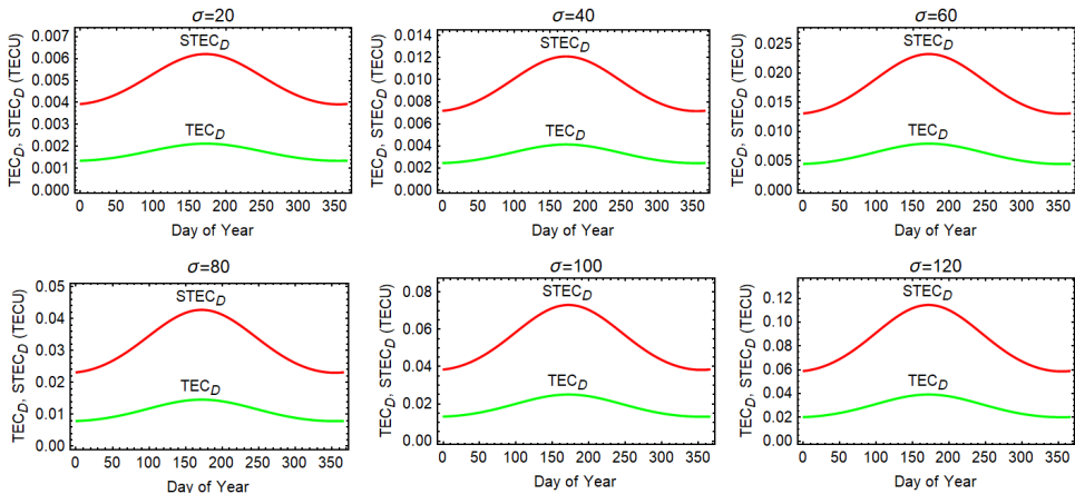
Fig. 3. Compared vertical and slant total electron content values in D-region over year for different \sigma values.
